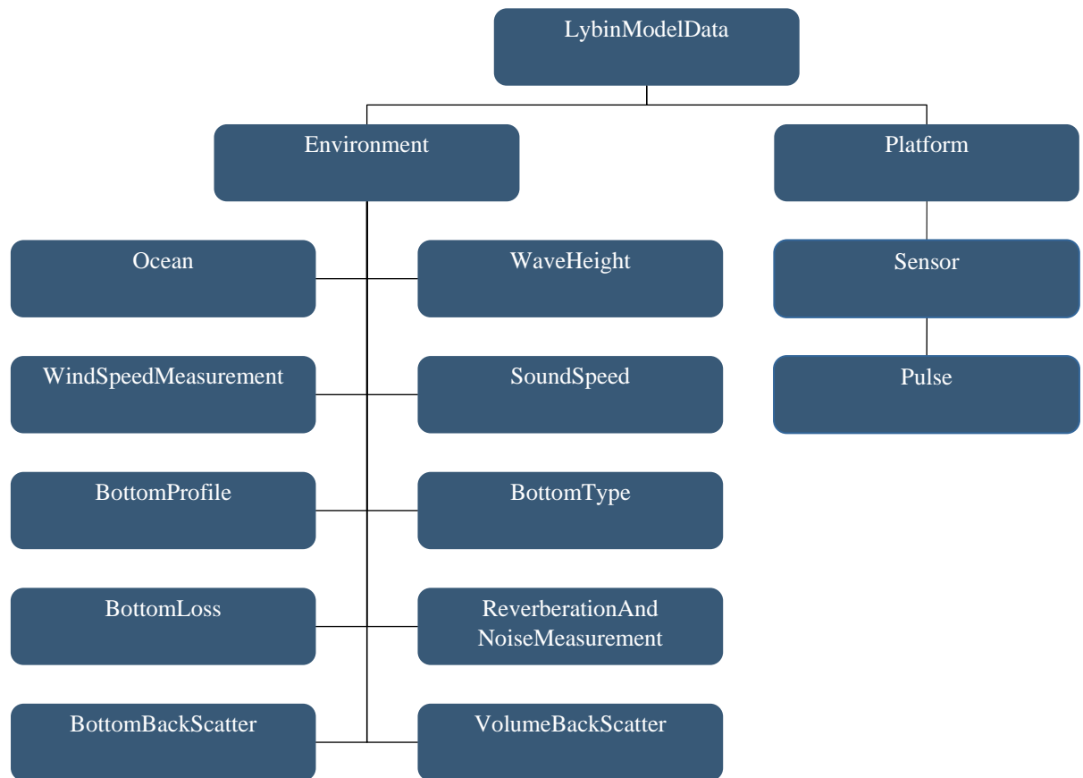
Figure 2.2 The LybinCom input data model (Class diagram).
